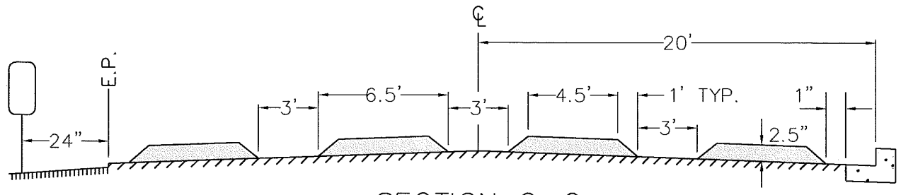
SECTION C-C
