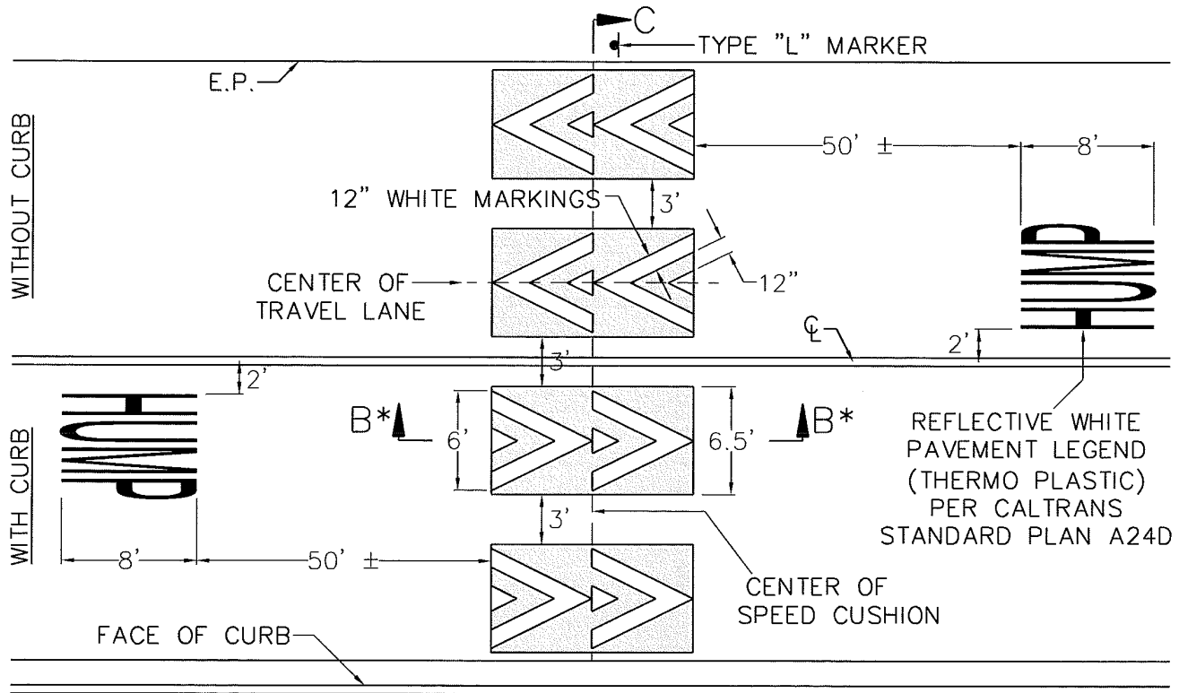
PLAN VIEW
