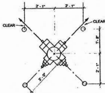
BARRICADE PLACEMENT (WHEN SPECIFIED)
