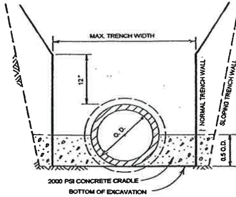
CRADLE FOR EXCESSIVE TRENCH BOTTOM WIDTH - L. F. 2.3
