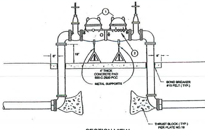
SECTION VIEW
