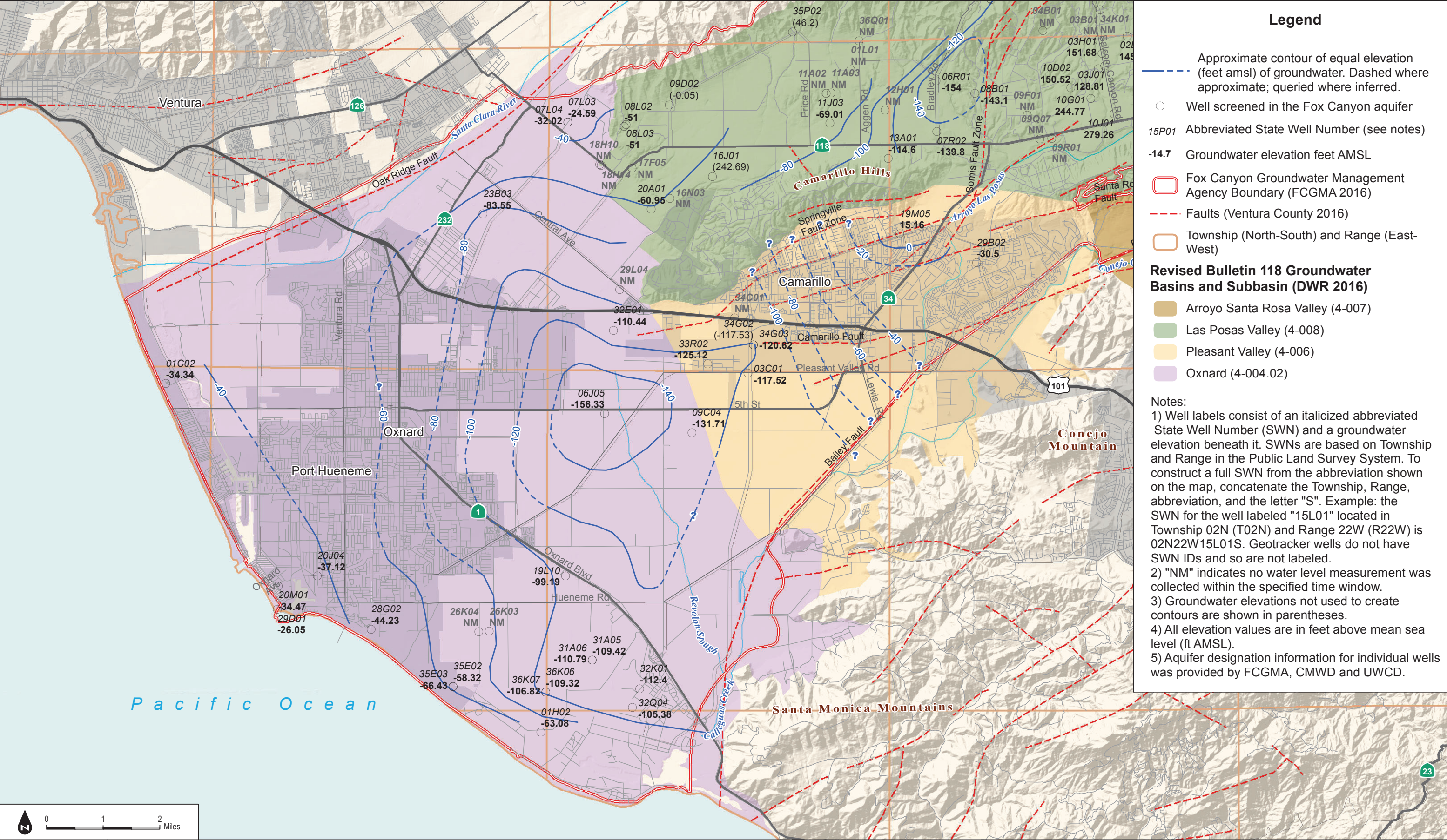
FIGURE 2-15 Groundwater Elevation Contours in the Fox Canyon Aquifer, October 2-29, 2015
