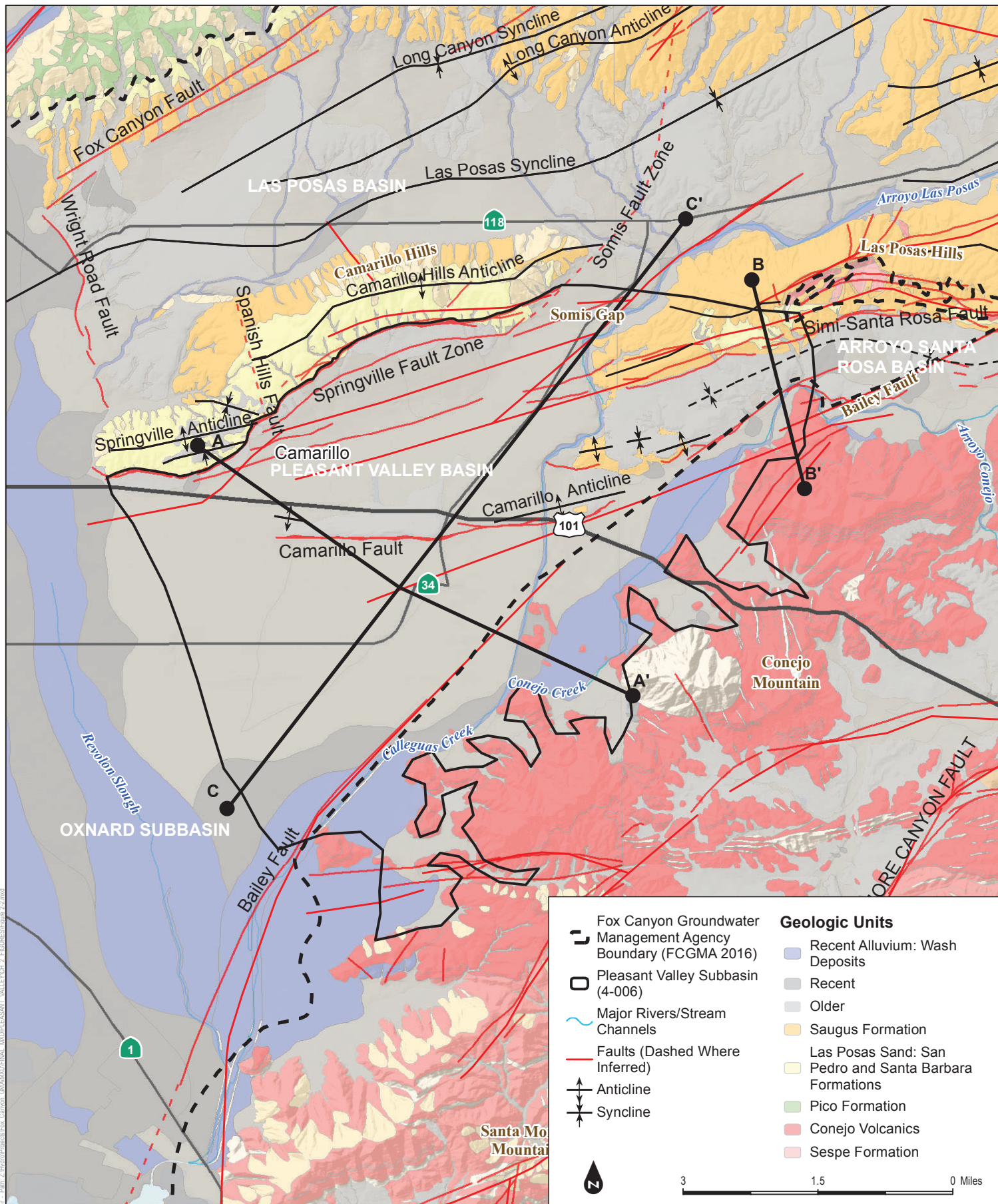
FIGURE 2-2 Geology of the Pleasant Valley Basin
