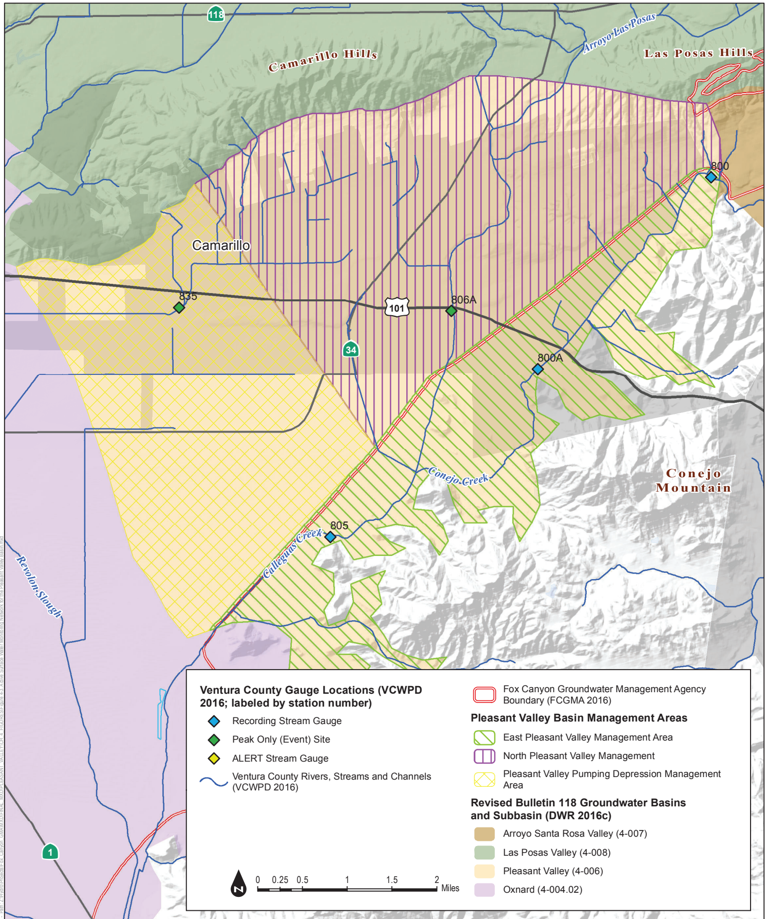
FIGURE 4-3 Active Surface Water Monitoring Network for the Pleasant Valley Basin
