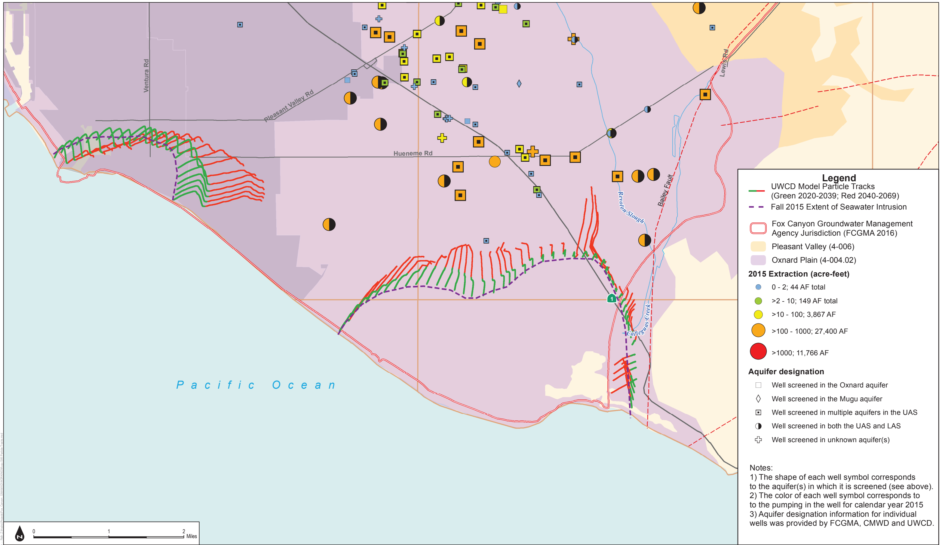
Figure 2-64b UWCD Model Particle Tracks, Mugu Aquifer, Future Baseline
