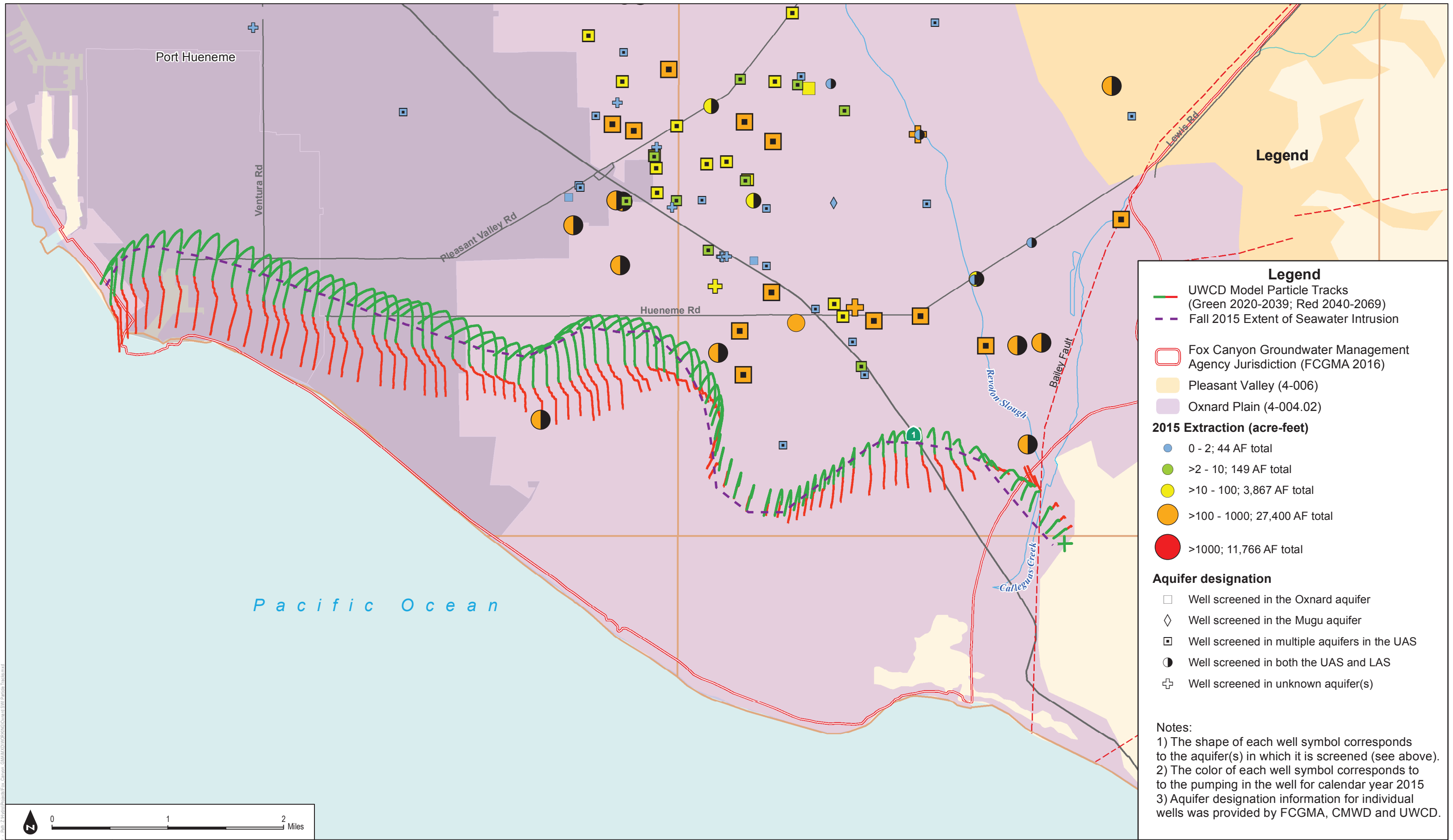
Figure 2-68a UWCD Model Particle Tracks, Oxnard Aquifer, Reduction Without Projects Simulation 1 - 27,200 AFY Groundwater Production in the UAS
