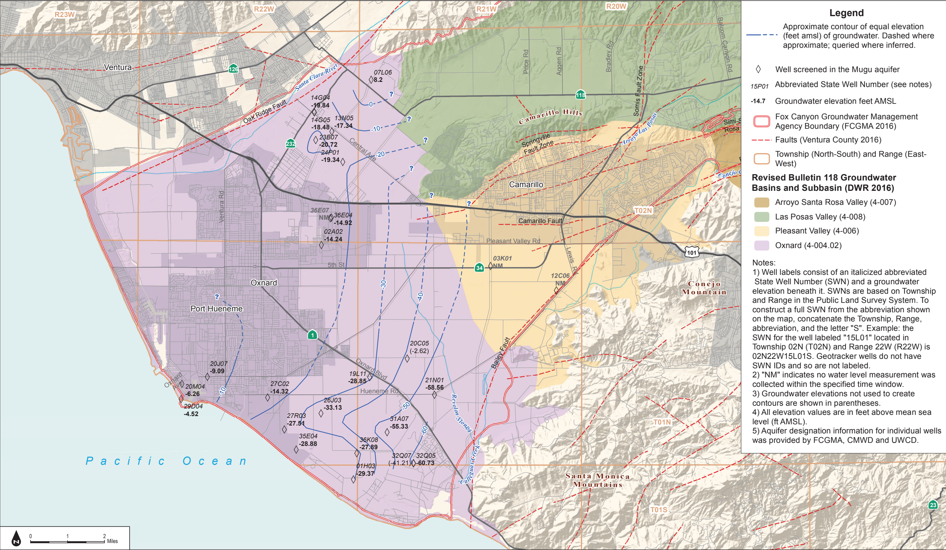
FIGURE 2-10 Groundwater Elevation Contours in the Mugu Aquifer, March 2-29, 2015
