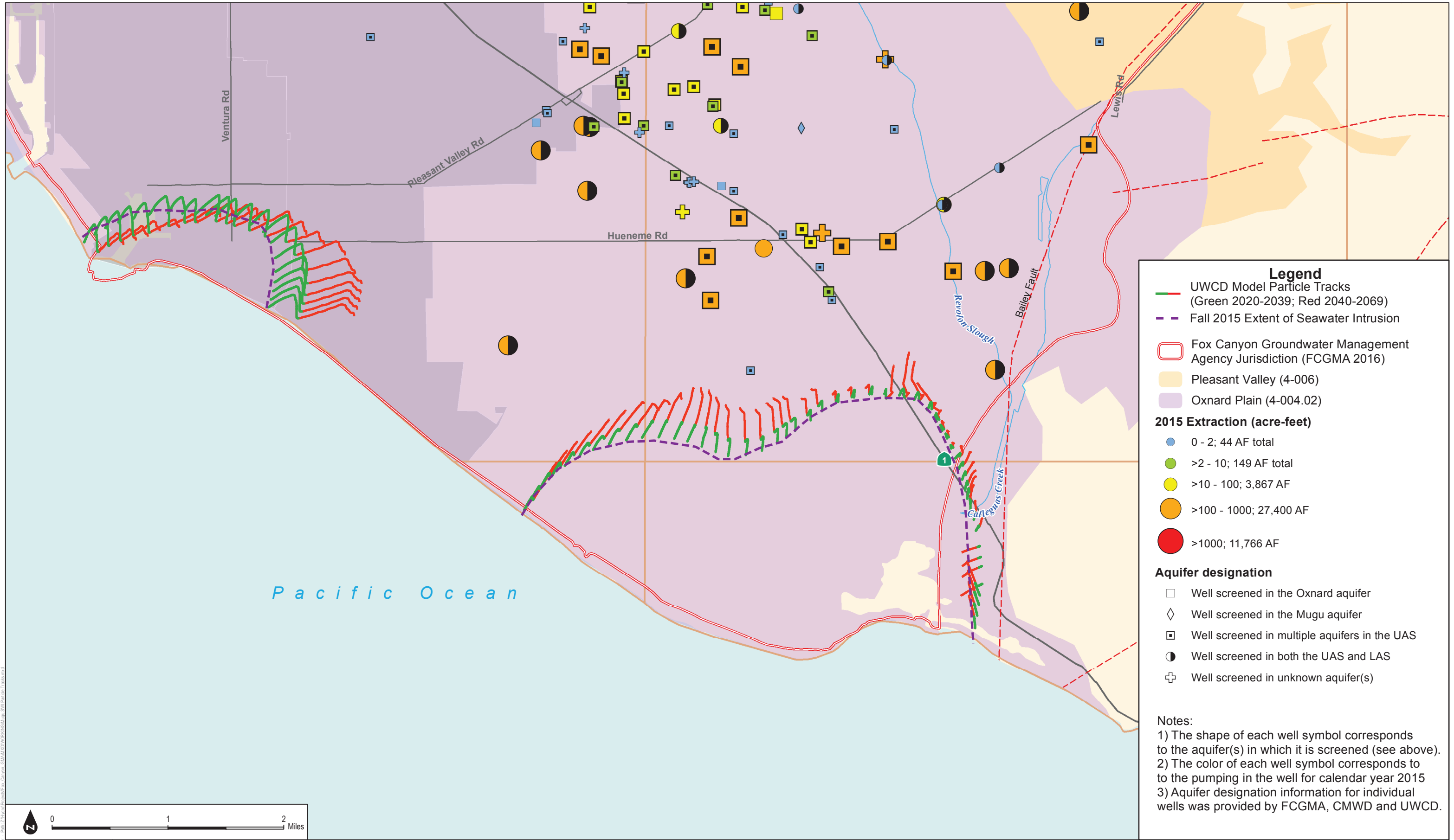
Figure 2-66b UWCD Model Particle Tracks, Mugu Aquifer, Future Baseline With Projects
