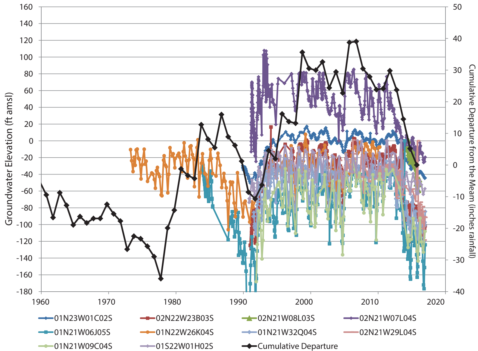
FIGURE 2-18 Groundwater Well Hydrographs in the Fox Canyon Aquifer
