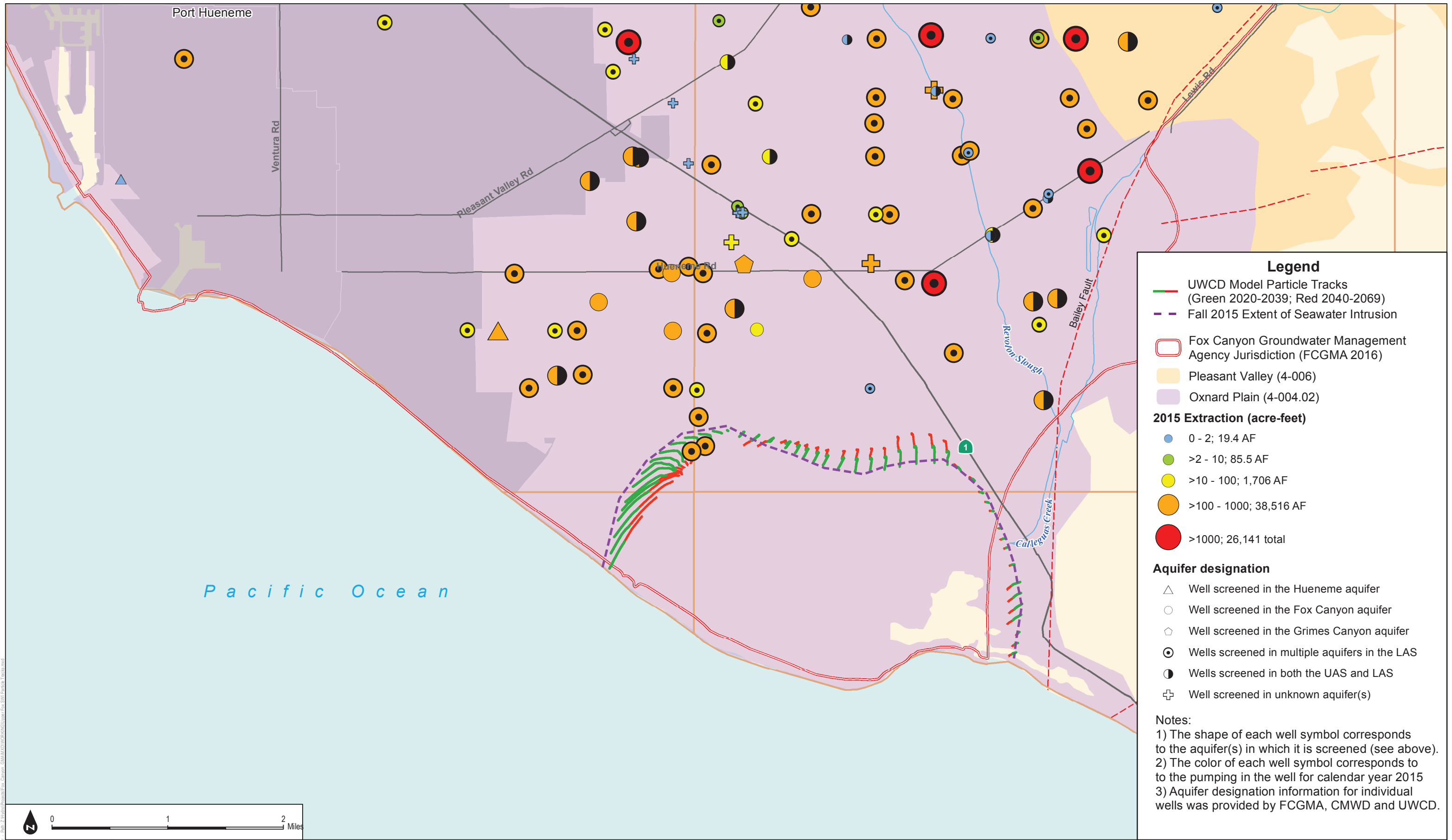
Figure 2-67d UWCD Model Particle Tracks, Upper Fox Canyon Aquifer, Reduction with Projects Simulation - 12,800 AFY Groundwater Production in the LAS
