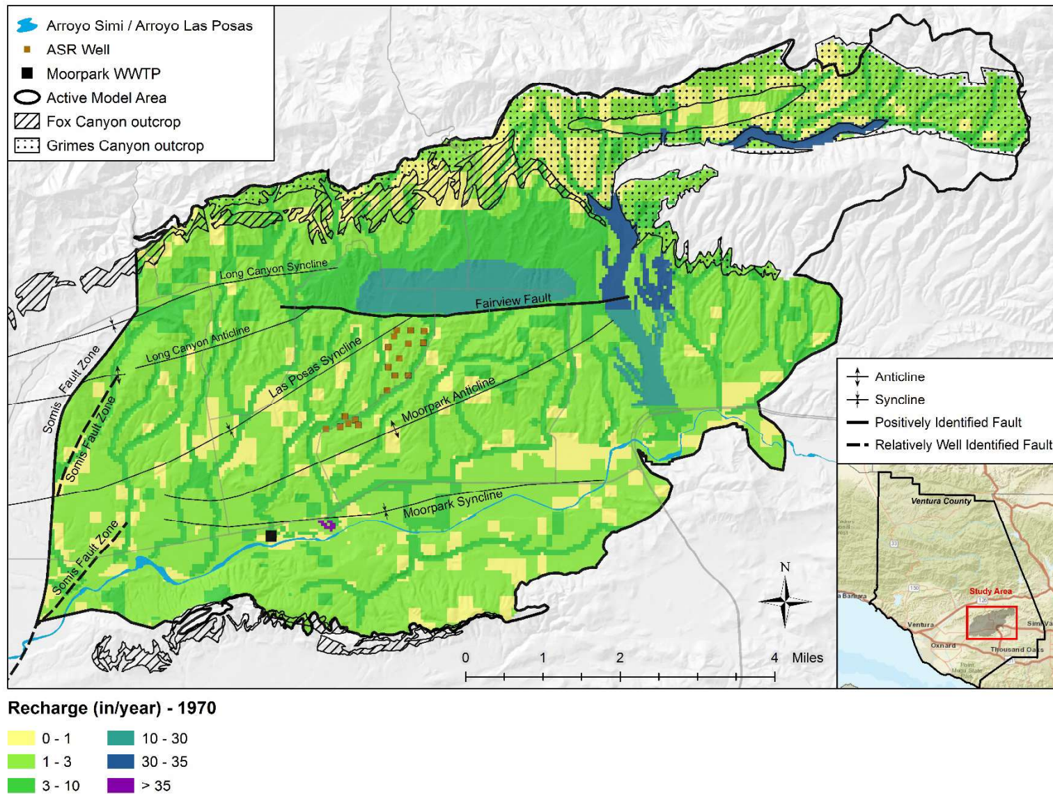
Figure 8-6 Recharge (in/year) for January, 1970
