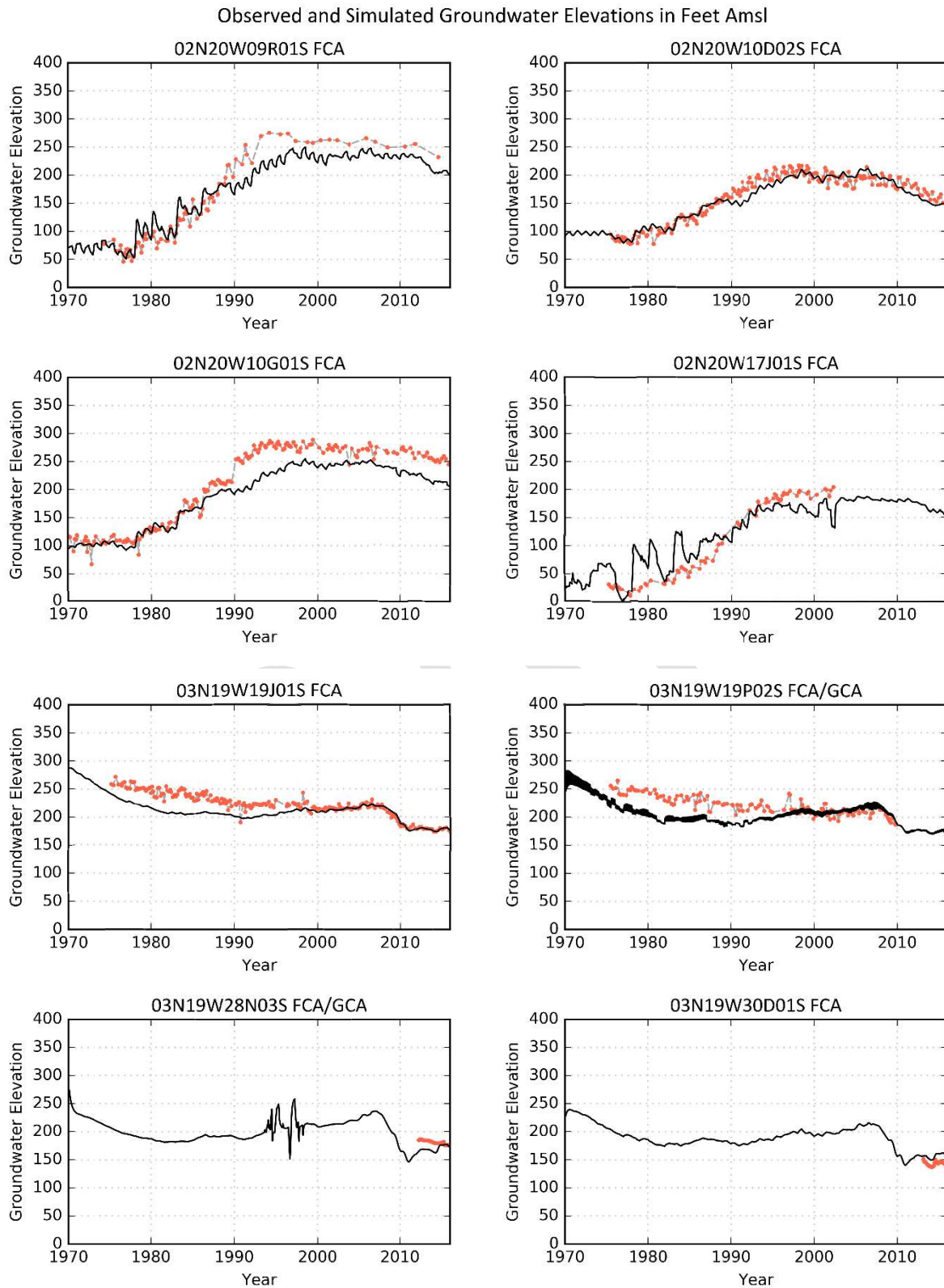
Figure 8-62b Simulated versus observed hydrographs at key wells in the FCA (Layer 5)
