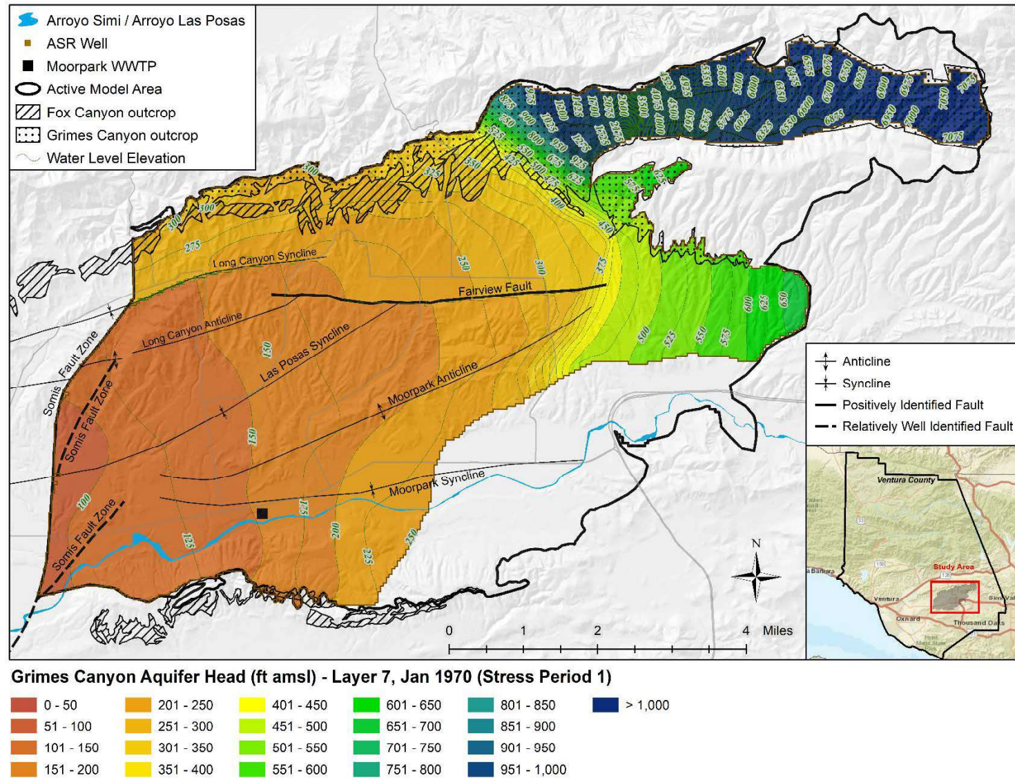
Figure 8-55 Layer 7 (GCA) hydraulic heads (ft amsl) – Jan 1970 (Stress Period 1)
