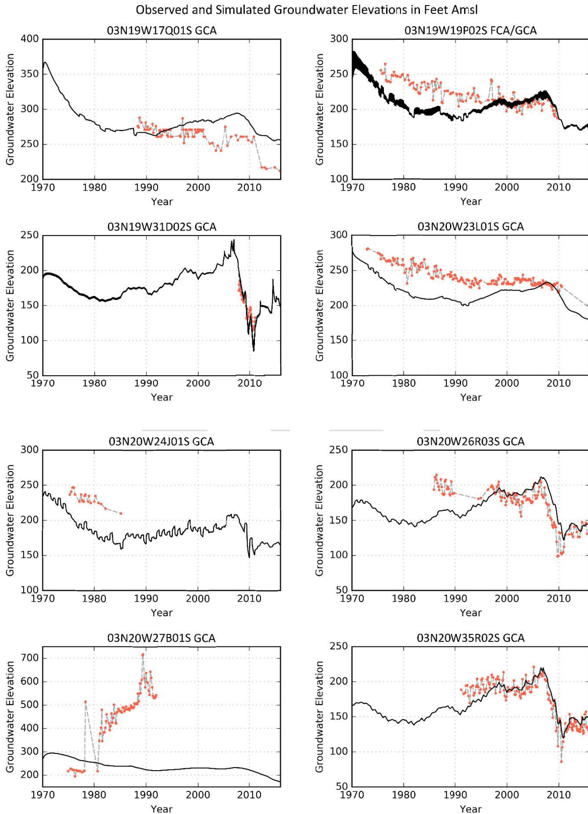
Figure 8-63 Simulated versus observed hydrographs at key wells in the GCA (Layer 7)
