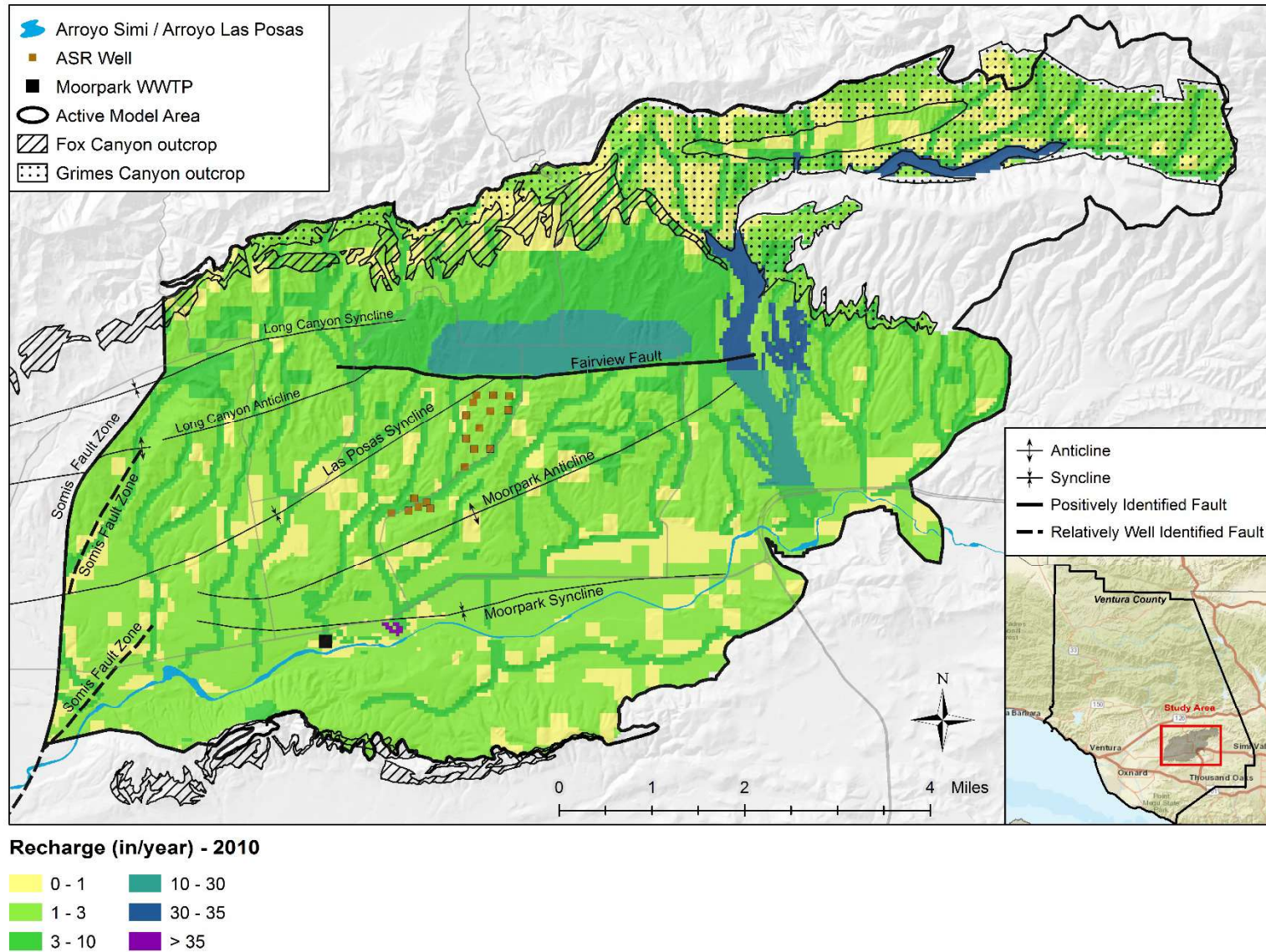
Figure 8-7 Recharge (in/year) for January, 2010
