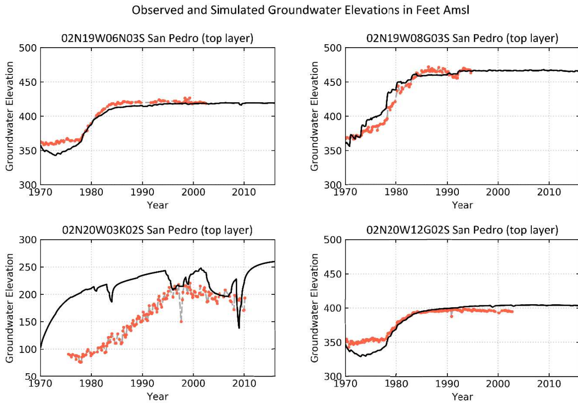
Figure 8-60 Simulated versus observed hydrographs at key wells in the Top Layer of the Upper San Pedro/Saugus Formation (Layer 2)
