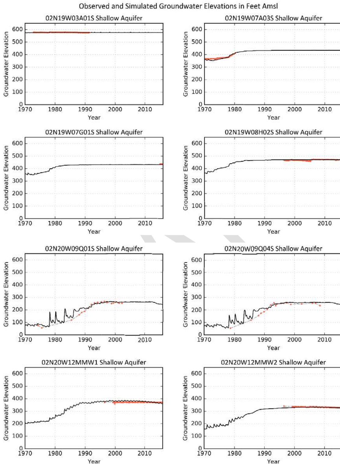
Figure 8-58 Simulated versus observed hydrographs at key wells in the Shallow Aquifer (Layer 1)
